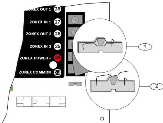
Figure 2.3: Reset Pin
