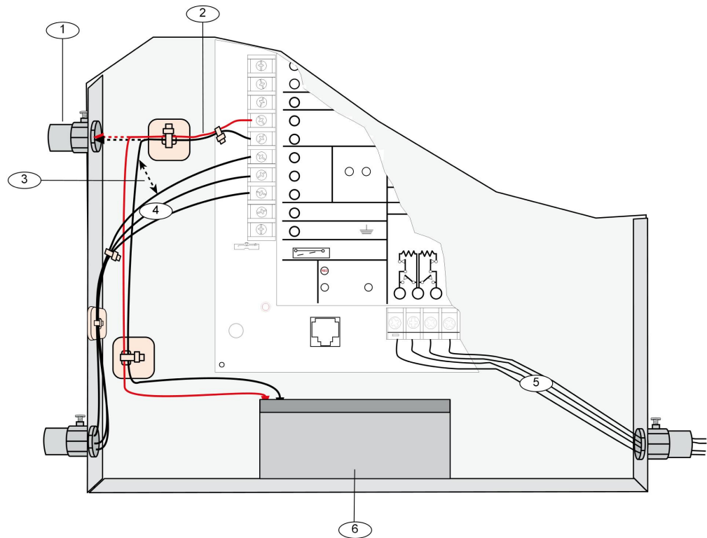
Figure 4.14: Non-PowerLimited Wiring
