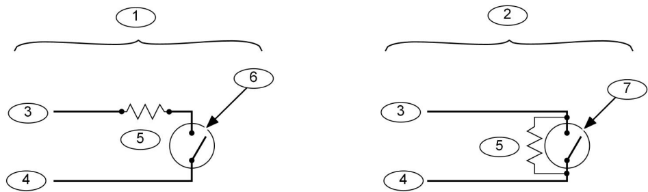
Figure 3.12: Keyswitch Wiring
